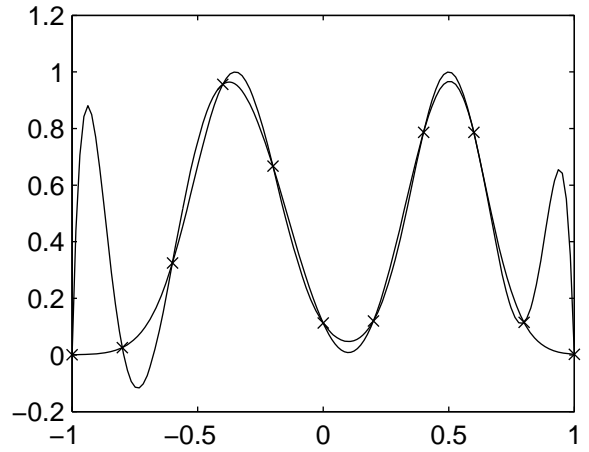
Lanrange poly of degree 10
