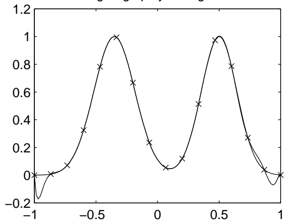
Lanrange poly of degree 15
