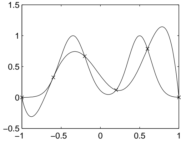
Lanrange poly of degree 5
