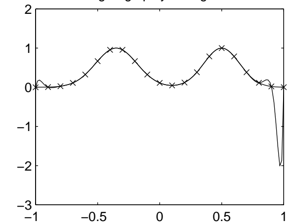
Lanrange poly of degree 20
